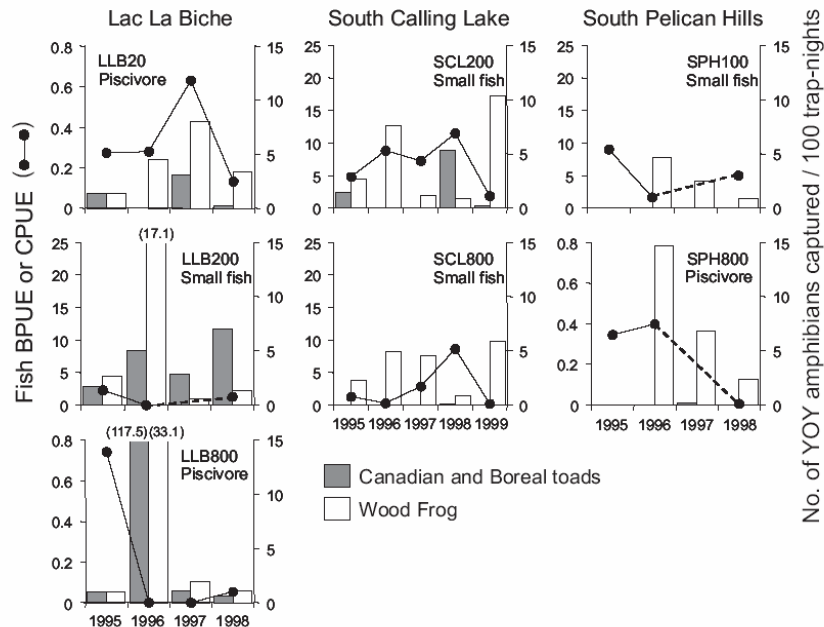
Fig. 1. Abundance of fish and young-of-the-year (YOY) Wood Frog ( Rana sylvatica ) and toads (Boreal, Bufo boreas boreas , and Canadian, Bufo hemiophys , toads combined) from the seven study lakes in three regions of boreal Alberta. Fish communities are classified as being dominated by larger, piscivorous species or by small species. Abundance estimates for fish are in biomass per unit effort (BPUE, kg-h -1 ; piscivores) or catch per unit effort (CPUE, number of fish captured-h -1 ; small fish); amphibian estimates are in CPUE (numbers / 100 trap-nights). Amphibians were not sampled at the SPH lakes in 1995; fish were not sampled in 1997 at LLB200 or the SPH lakes.
